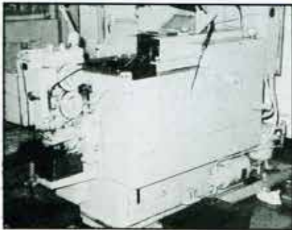
3/16" National High Speed DSSD Cold Header
