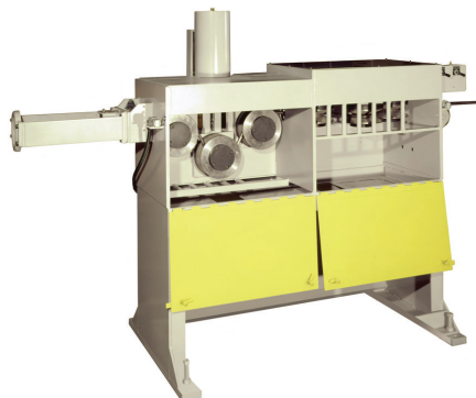
Mechanical Descaler For Hot Rolled Rod
