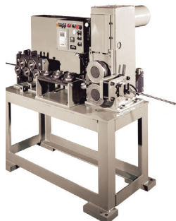
Power Feed & Straighteners
