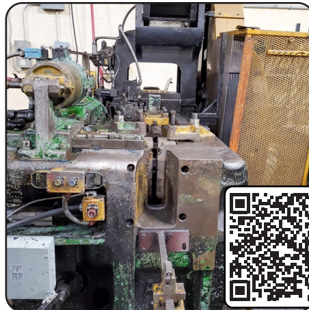
1-1/2" AJAX Upsetter w/ Air Clutch Ref. No. 26609
