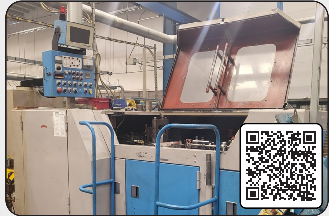
3/8" Asahi Okuma AOS-10-15 2 Die 2 Blow Ref. No. 26691
