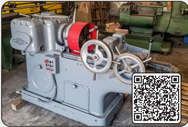
2" Landis Single Spindle with Lead Screw Ref. No. 25550
