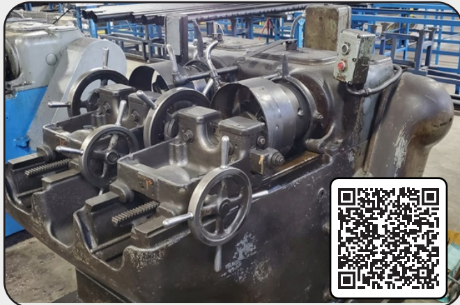
1-1/2" Landis Double Spindle Thread Cutter Ref. No. 26615
